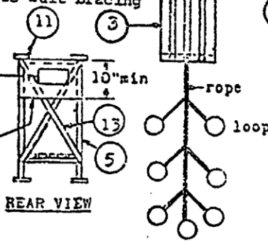
TOWING BRIDLE
